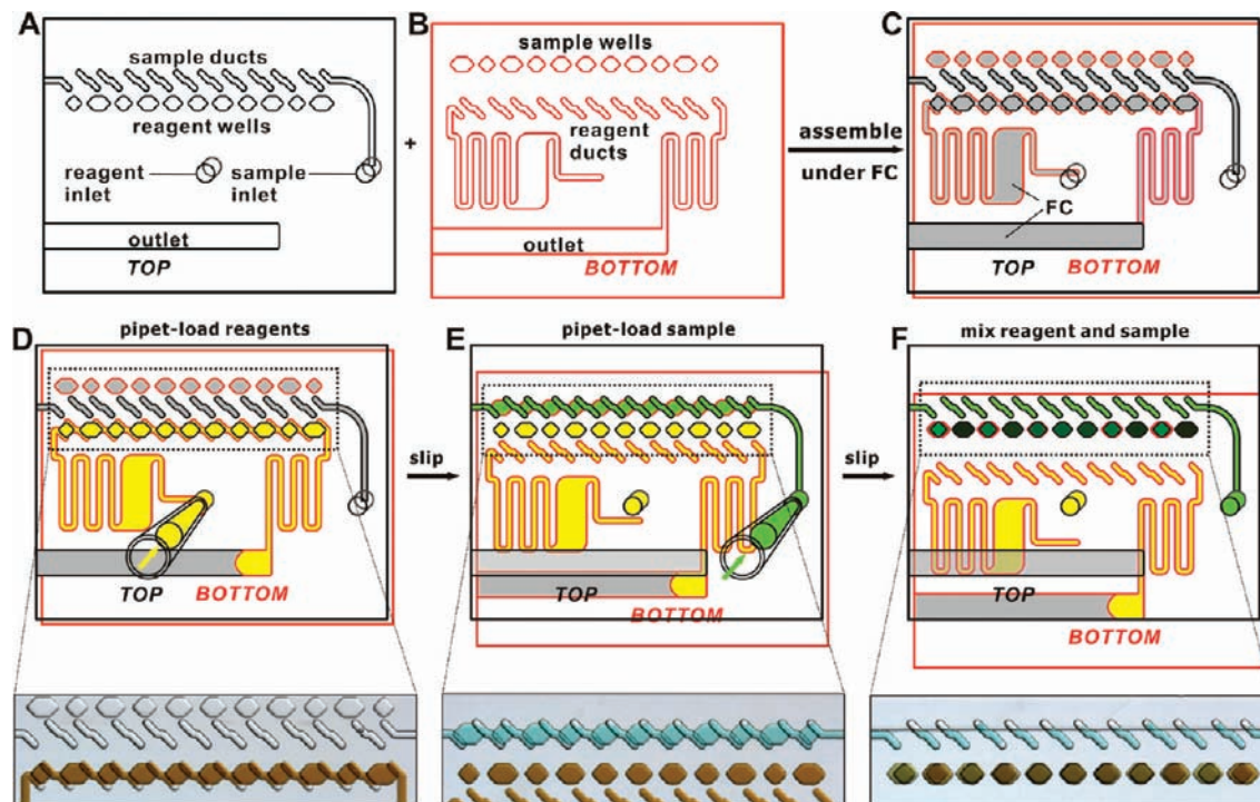
Figure 3. A zoomed-in schematic of the area outlined in Figure 2B and corresponding experimental microphotographs showing the operation of the user-loaded SlipChip (see supporting movie S2). (A) The top plate (contoured in black) consisted of an outlet channel, a reagent inlet, a sample inlet aligned to sample ducts, and reagent wells. (B) The bottom plate (contoured in red) consisted of an outlet aligned with reagent ducts and sample wells. (C) The top plate and bottom plate were assembled and filled with fluorocarbon to generate a SlipChip ready for use. In this orientation, a continuous fluidic path was formed by the reagent inlet, the reagent wells, and the outlet. (D) A reagent was introduced by pipetting. The reagent (yellow) flowed through the continuous fluidic path and filled the reagent wells. A microphotograph below the schematic shows brown dye solution being loaded as the reagent. (E) The chip was slipped into a second position. In this second position, a continuous fluidic path was formed by the sample inlet, the sample ducts, and the sample wells. The sample (green) was introduced by pipetting. The sample flowed through the continuous fluidic path and filled the sample wells. A microphotograph below the schematic shows green dye solution being loaded as the sample. (F) The chip was slipped again into the third position, where the reagent wells were aligned on top of the sample wells, and the sample and reagent in the aligned wells combined by diffusion (dark green). A microphotograph below the schematic shows the reagent combining with the sample in each well, forming individual experiments. The colors of the reagent and the sample in D–F are not consistent for the schematics and the microphotographs. The colors in the schematic were changed to better illustrate the operation of the SlipChip.
