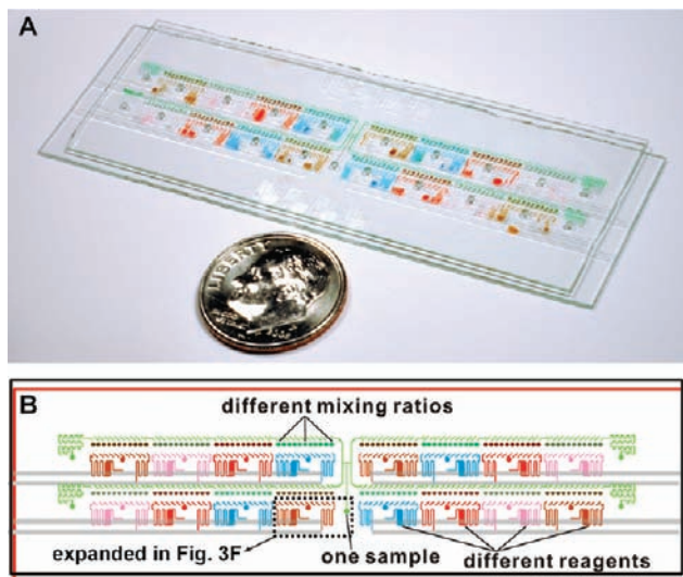
Figure 2. A user-loaded SlipChip to screen one sample (green) against 16 different reagents (shown with other colors) at different concentrations. (A) A photograph of the SlipChip fabricated in glass with fluid paths filled with food dyes (US dime is shown for scale). (B) A schematic of the layout of the user-loaded SlipChip, expanded and operation explained in Figure 3.
