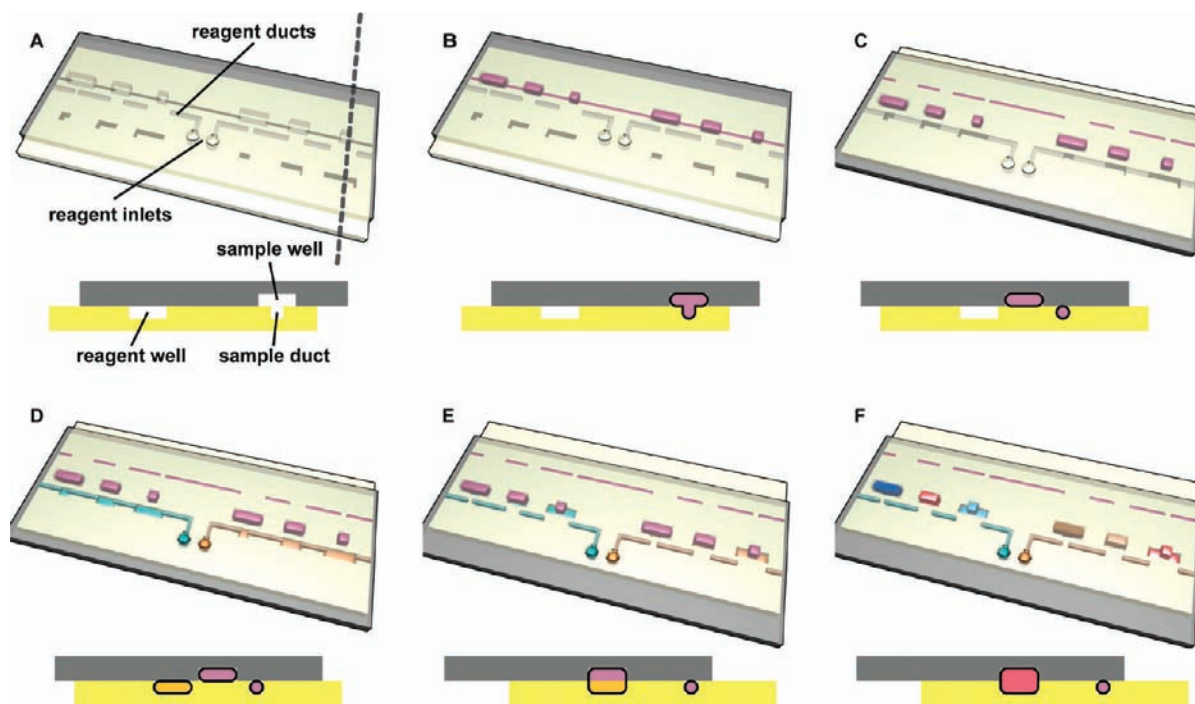
Figure 1. Step-by-step 3D schematic drawings with cross-sectional views that describe the operation of a user-loaded SlipChip. (A) In the starting orientation, the two plates of the SlipChip are aligned such that the sample wells and sample ducts are aligned to form a continuous fluidic path, and the reagent wells and reagent ducts are offset. (B) The sample (purple) is loaded through the continuous fluidic path formed by overlapping sample wells (top plate) with sample ducts (bottom plate). (C) The device is slipped such that the reagent wells (bottom plate) and reagent ducts (top plate) are now aligned. (D) Reagents (blue and yellow) are loaded into the individual fluidic paths formed by overlapping reagent wells and sample wells. (E) The device is slipped a second time, and the sample wells from the top plate are exposed to the reagent wells of the bottom plate. (F) The pink well schematically shows a reaction taking place after mixing and incubation (see movie S1).
